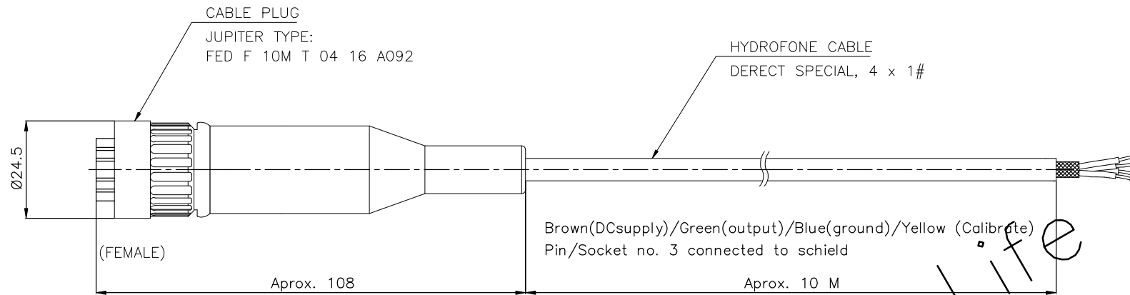
ELECTRICAL WIRING DIAGRAM
